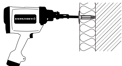
2] Push the pinner all the way into the insulation. Support the back of the pinner with the palm of your free hand.
